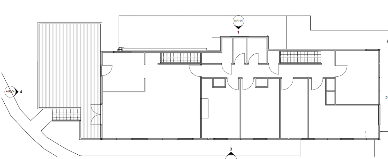
3 Top Floor (Existing) 1 : 100
