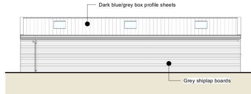
5 West - Proposed 1 : 100
