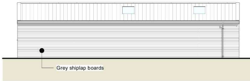
2 East - Proposed 1 : 100
