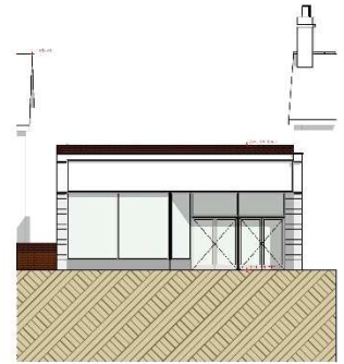
5 Existing Front Elevation 1:100
