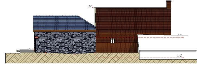
1 Existing Side Elevation 1:100
