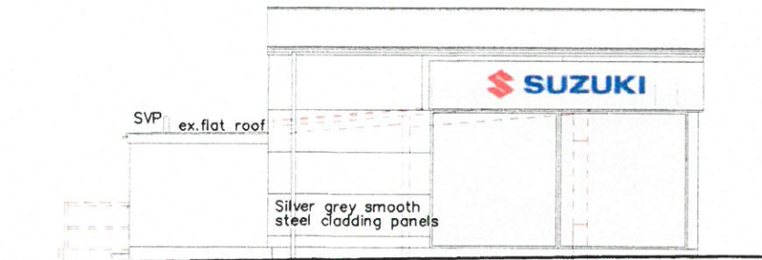
SIDE ELEVATION
