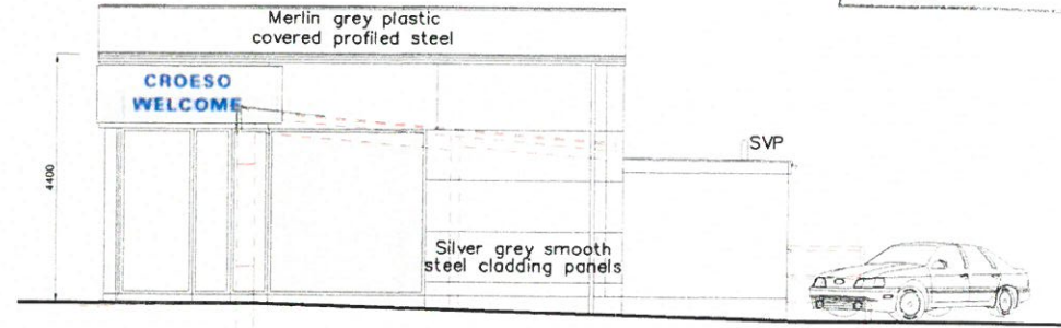
SIDE ELEVATION
