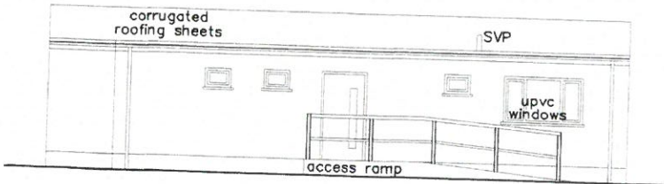
REAR ELEVATION
